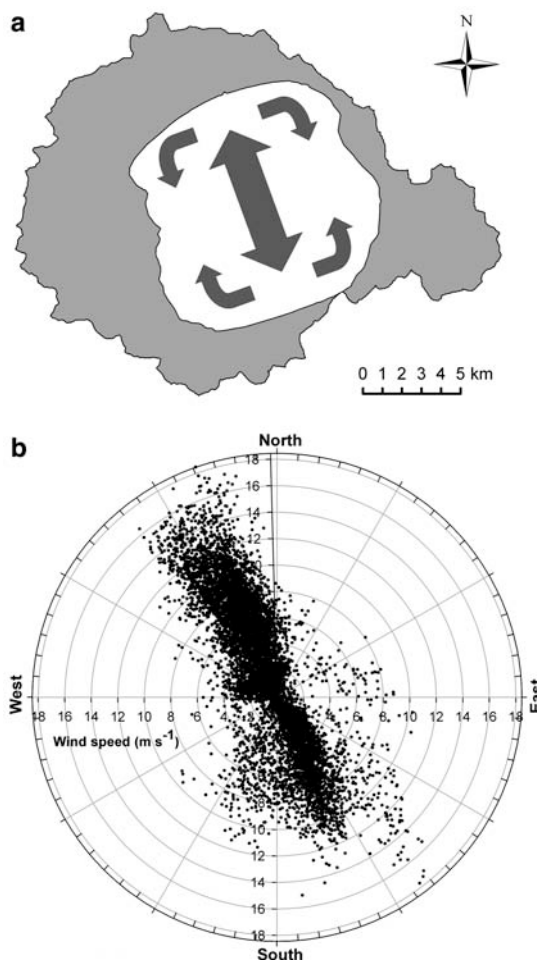
Fig. 5 Surface water dynamics schematic (a) and 2002 hourly wind speeds and directions (b). The orientation of the lake is identical to the dominant wind direction (bearing 335 degrees) to within the measurement accuracy of 5°. How winds help shape the lake is described in the text
