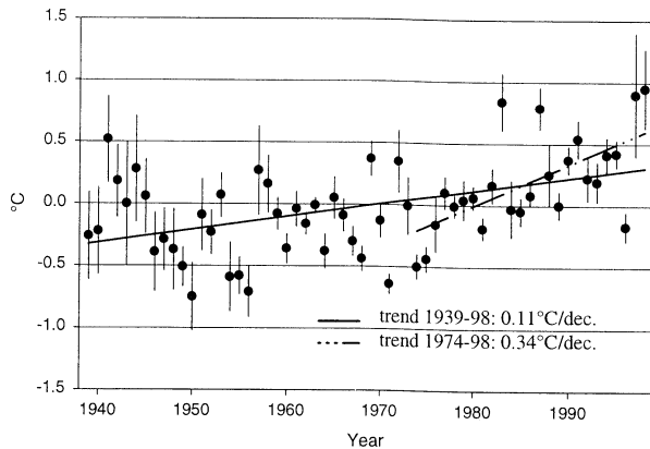
Figure 3. Annual temperature deviation from the 1961-1990 average in the tropical Andes (1°N-23°S) between 1939 and 1998. Trend estimates are based on ordinary least squares (OLS) regression. Vertical bars extend 2 standard errors of the mean either side of the annual average.
