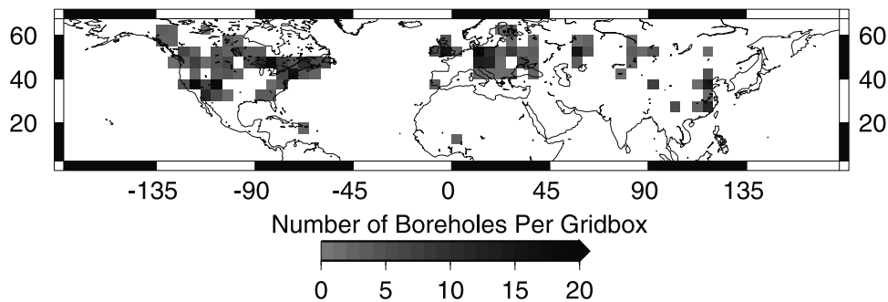
Figure 1. Distribution of the Northern Hemisphere borehole temperature reconstructions. The locations of the (94) 5 by 5 grid points sampled by the individual borehole reconstructions of HPS00 are shown, along with density of samples contributing to each grid point.
