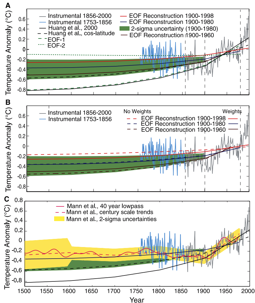
Figure 6. Borehole-based reconstructions of Northern Hemisphere mean temperature compared with instrumental Northern Hemisphere annual mean surface temperature ( Jones et al. [1999]; light gray) extended to mid 18th century with the available instrumental data (see text; light blue-gray). (a) HPS00 Northern Hemisphere temperature reconstruction compared to areally weighted mean of gridded HPS00 borehole reconstructions, and optimal borehole hemispheric SAT estimate (using 1900–1960, 1900–1980, and 1900–1998 projection intervals). The 95% confidence interval (light green shading) is also shown for the reconstruction corresponding to the 1900–1980 projection interval. Also shown are the separate projections of the first two eigenvectors onto hemispheric mean temperature. (b) Comparison of the optimal borehole SAT estimate for the unweighted and weighted borehole grid point GST reconstructions. (c) Comparison of HPS00 reconstruction, areally weighted mean of gridded HPS00 borehole reconstructions, and the optimal borehole estimate (based on 1900–1980 target instrumental signal; 95% confidence interval also shown) with Mann et al. [1999] reconstruction (latter shown both as smoothed (40 year lowpassed) annual values, and piecewise continuous linear trend estimate with its associated 95% confidence interval).
