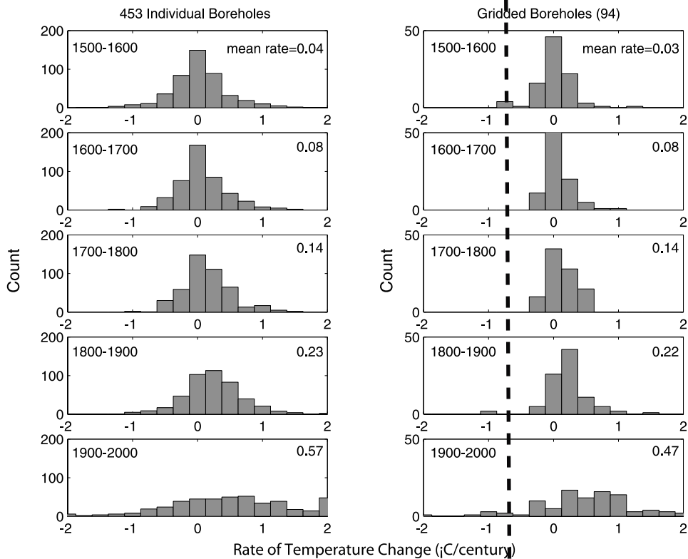
Figure 2. Histogram of distribution of trends among the (a) 453 individual and (b) gridded Northern Hemisphere borehole reconstructions for each of the past five centuries. Mean rates of change are indicated for each century in both cases.
