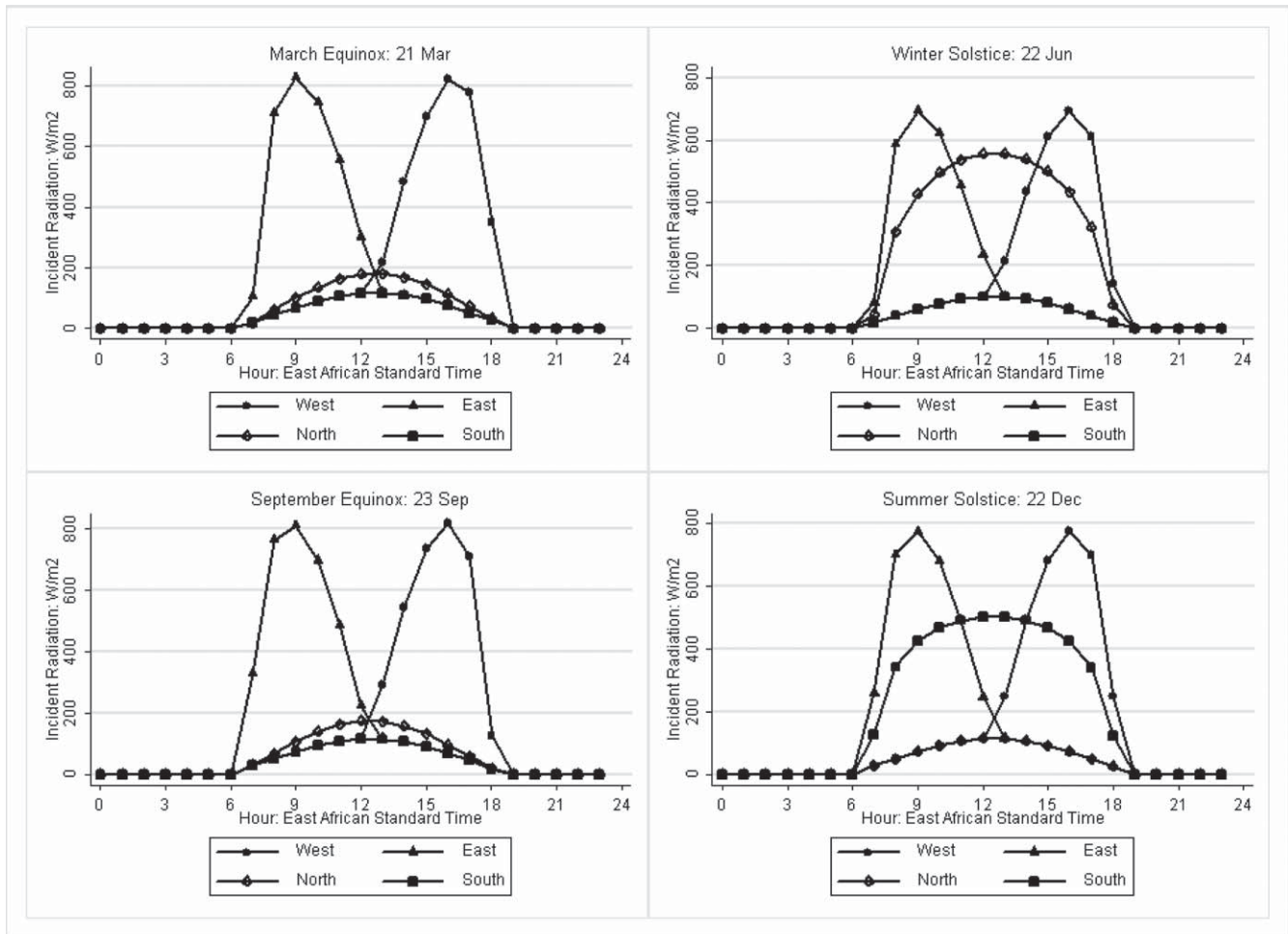
FIGURE 7. Modeled solar radiation ( W/m^2 ) received on vertical walls facing north, south, east, and west at the four main seasons (equinoxes and solstices) for Kilimanjaro. Note how north/south-facing walls receive substantial radiation only during the solstice period when the sun is in the appropriate hemisphere (one season out of four).
