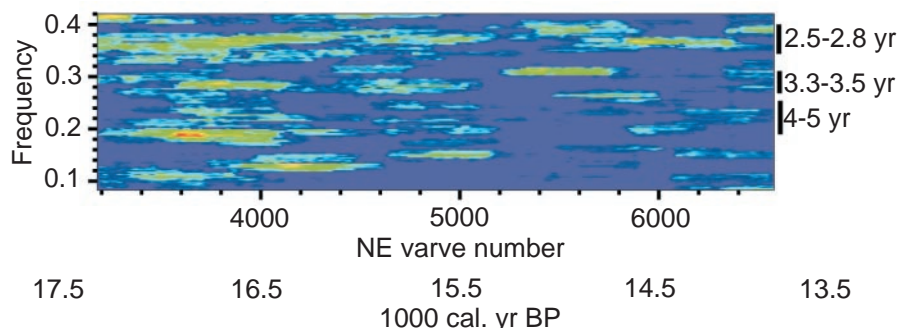
Fig. 4. Evolutionary spectral analysis from the NE varve chronology data set (NE varve numbers 2868 through 6900) covering the interval from 17,500 to 13,500 cal yr B.P. The spectrum is normalized everywhere by the median red noise level, so that the amplitude shown is proportional to the associated level of statistical significance. The background color is set to the median red noise level (50% confidence), and features evident above the background are significant at the >50% confidence level, with the lightest features being the most significant.
