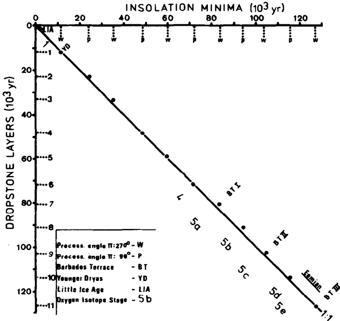
FIG. 7. Relationship of dropstone ages (from Fig. 6) and times of insolation minima (from Vernekar, 1972).
