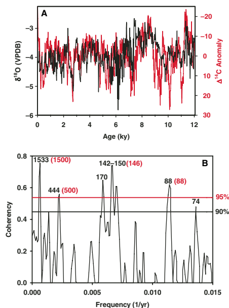
Figure 3. A: Covariation of raw \delta^{18}\text{O} record (black line) and detrended \Delta^{14}\text{C} data (INTCAL 98) (red line) (Stuiver et al., 1998). We detrended \Delta^{14}\text{C} data by subtracting six degree polynomial long-term trend from data. Scales for two records are in opposite direction to each other to show negative correlation. In this case, higher \delta^{18}\text{O} values correspond to lower \Delta^{14}\text{C} values but higher solar intensity. Zero reference is A.D. 1955. Two records have excellent visual match. Correlation coefficient for two records for entire Holocene is R = -0.34 to -0.38 (20–50 yr interpolation). We do not know cause of mismatch ca. 7.2 ka. B: Cross-spectral analysis, using computer package SPECTRUM (Schulz and Stettger, 1997), of raw \delta^{18}\text{O} and raw \Delta^{14}\text{C} time series. Parameters for coherency calculations were similar to those used for univariate spectral analysis (Fig. 2B). 95% and 90% false alarm limits are shown as solid and dashed lines, respectively. Significant peaks (in black) include 1533, 444, 170, 146, and 88 yr. Corresponding numbers in red are peaks previously associated with solar peaks (Sonnett and Finney, 1990; Stuiver and Braziunas, 1993). VPDB—Vienna Peedee belemnite.
