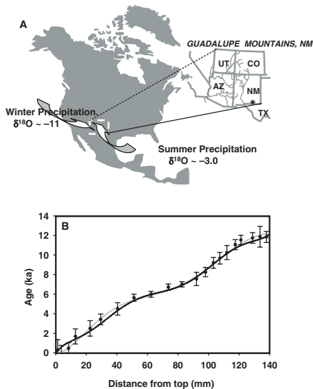
Figure 1. A: Guadalupe Mountains, New Mexico, site of Pink Panther Cave and typical of other parts of U.S. southwest, has two rainy seasons. Summer North American monsoon (NAM) rainfall (Adams and Comrie, 1997), derived from Gulf of Mexico, is characterized on average by heavy \delta^{18}\text{O} values ( \sim -3\% ), while winter Pacific-derived precipitation is characterized by low \delta^{18}\text{O} values ( \sim -11\% ) (Hoy and Gross, 1982; Yapp, 1985). B: Chronology of PP1, showing distance from top of stalagmite to bottom vs. U-Th ages. Solid curve is age model based on 9 degree polynomial fit of chronology data, covering entire period. Error bars reflect analytical errors, including uncertainties related to estimate of initial ^{230}\text{Th}/^{232}\text{Th} ratio (details on chronology, including analytical methods, are in Table DR1; see footnote 1).
