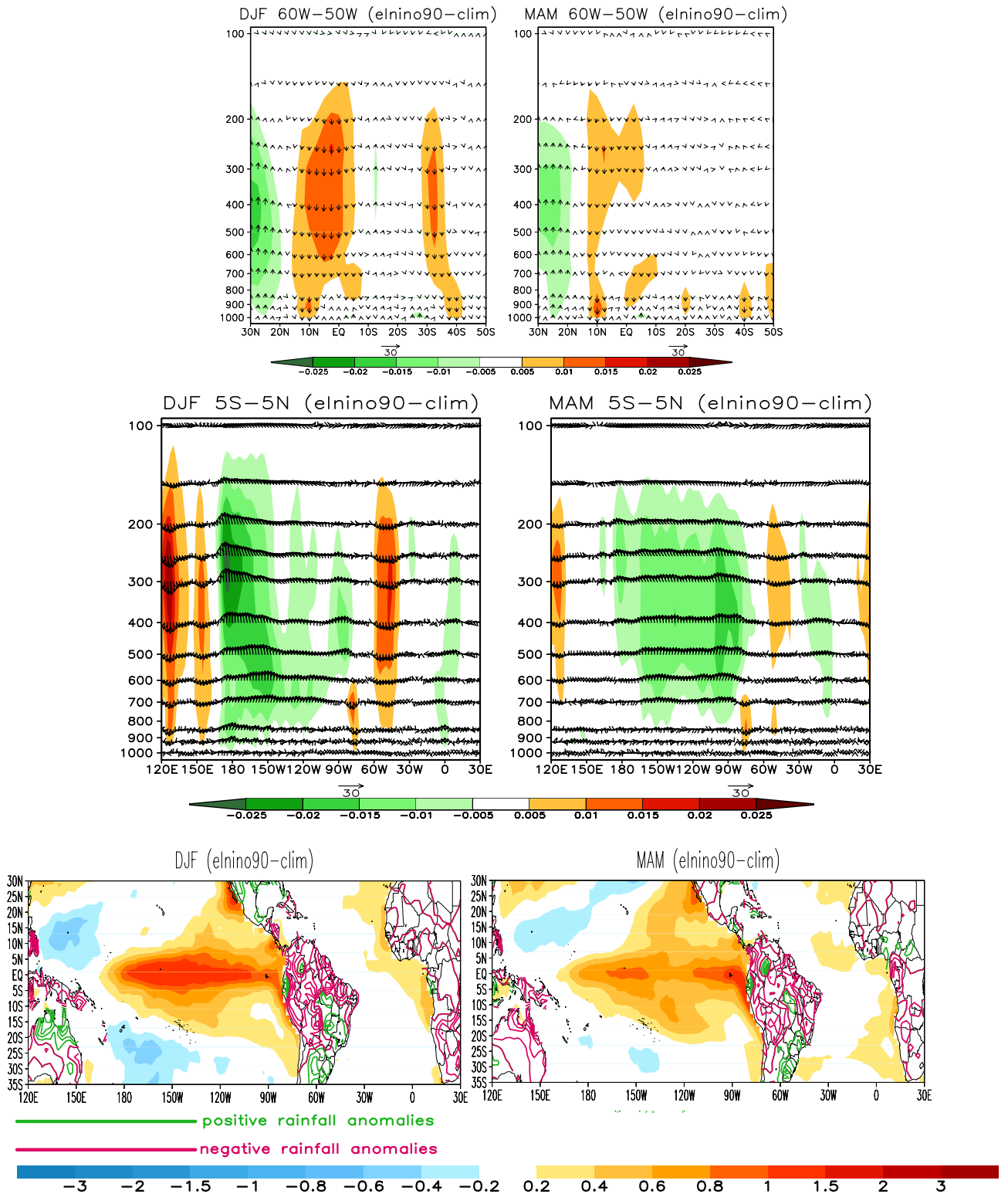
Figure 1: – Composite of El Niño episodes observed during the 1990s for the DJF (left) and MAM (right) seasons. Top figures are seasonal anomalies of omega (shaded) and meridional-vertical circulation (vectors). The intermediate figures are seasonal anomalies of omega (shaded) and zonal-vertical circulation. Lower figures show seasonal anomalies of SST (shaded) and precipitation (contours).
