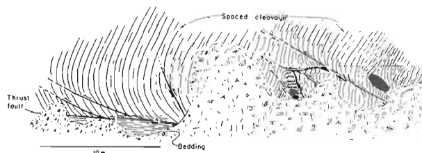
Fig. 9. Detail of cleavage drag against the floor thrust of the thick cleavage duplex and of imbricate thrusting that drags or displaces cleavage. See Fig. 8 for location.
