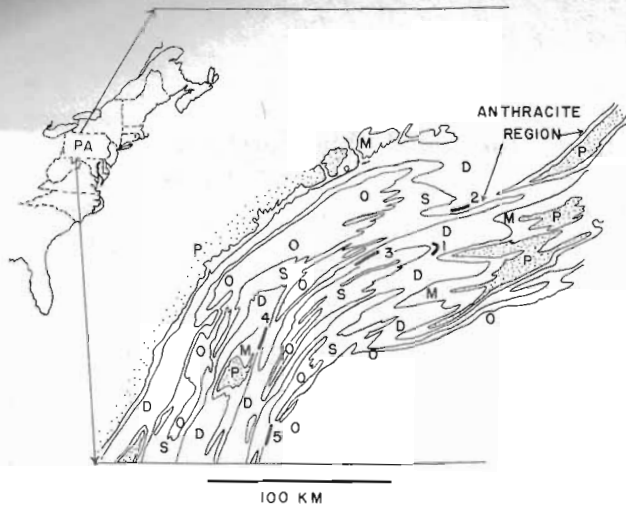
Fig. 1. Map of the Appalachian foreland (Valley and Ridge Province) in Pennsylvania. 1, 2, 3, 4 and 5 are cleavage duplex localities. 1, Selingsgrove Junction, Marcellus Formation; 2, Maudsley, Harrell Formation; 3, Bannerville, Harrell Formation; 4, Mapleton Depot, Marcellus Formation; 5, McConnellsburg, Reedsville Shale; O, Ordovician; S, Silurian; D, Devonian; M, Mississippian and P, Pennsylvanian.
