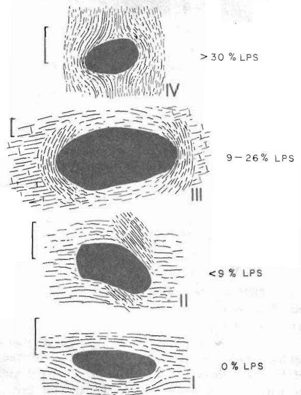
Fig. 10. Cleavage halo types I-IV and associated LPS (layer-parallel shortening). Scale bars are 10 cm long.
