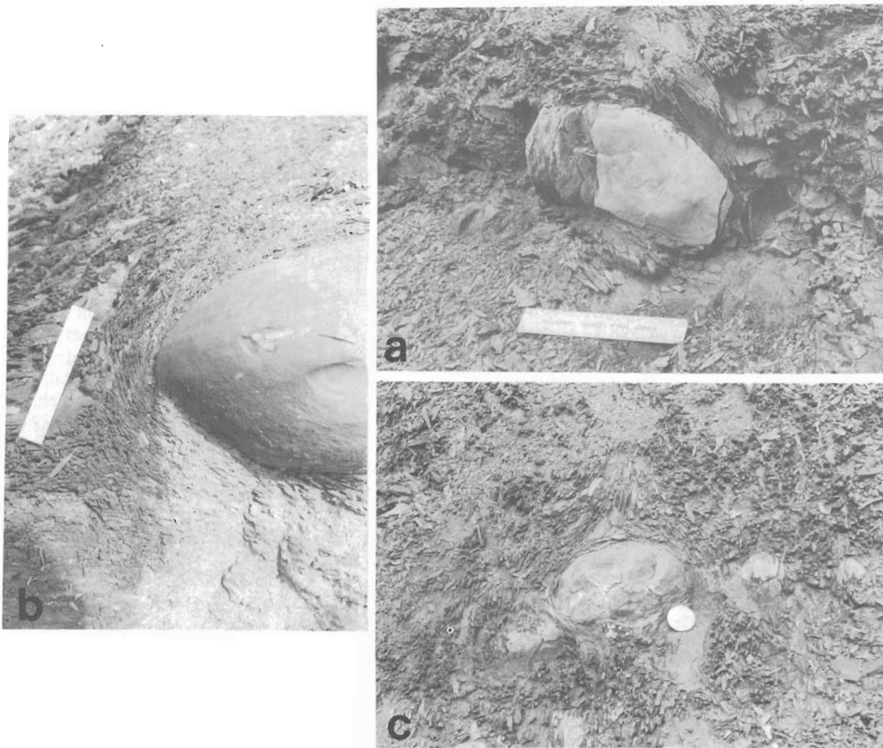
Fig. 11. Photographs of three types of cleavage halos around carbonate concretions. (a) Concretion with kink band or vertical cleavage zone, Type II scale 15 cm. Photographed in center of Fig. 12. (b) Concretion with platy cleavage zones at tips. Surrounding shale has pencil cleavage, Type III, scale 15 cm. Photographed at 210 m in Column 4, Fig. 3. (c) Concretion distorts pervasive spaced platy cleavage, Type IV, coin 23 mm. Photographed at lower right of Fig. 12.
