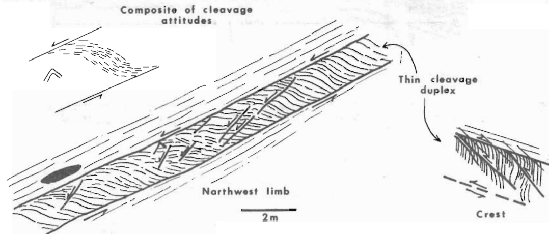
Fig. 5. Thin cleavage duplex on crest and northwest limb of Selinsgrove Junction second order anticline.
