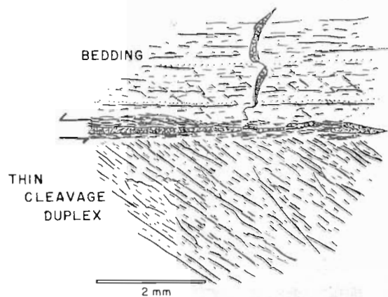
Fig. 6. Drawing of thin section across the roof of the thin cleavage duplex illustrated in Fig. 5. Granular quartz veins are parallel to the contact between bedding and the duplex and also cut bedding. Prominent S-planes are bedding, and, within duplex, spaced cleavage or transposed bedding.
