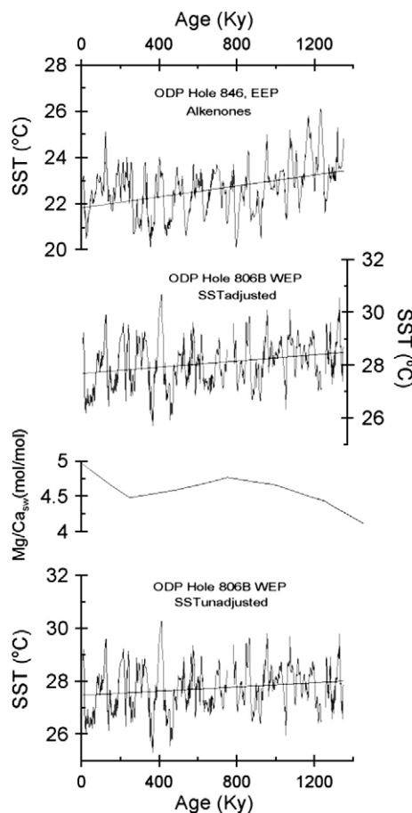
Fig. 8. EEP cold tongue and WEP warm pool SST records for the last 1.3 Ma. (A) ODP Hole 846 alkenone-based SST record (Liu and Herbert, 2004). (B) ODP Hole 806B WEP warm pool adjusted SST record based on Mg/Ca from the planktonic foraminifer Globigerinoides ruber (Medina-Elizalde and Lea, 2005). (C) FD06 seawater Mg/Ca reconstruction. (D) ODP Hole 806B unadjusted WEP warm pool SST record based on the planktonic foraminifer G. ruber (Medina-Elizalde and Lea, 2005). The adjusted WEP warm pool SST record suggests a cooling of ~1 °C similar to that implied for the EEP cold tongue by the ODP Hole 846 alkenone-SST record.
