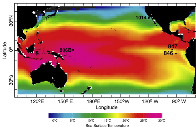
Fig. 2. Eastern and western Pacific Ocean Drilling Program (ODP) Site locations: western equatorial Pacific (WEP) warm pool ODP Hole 806B (0°N, 159°E, 2520-m water depth), eastern equatorial Pacific (EEP) cold tongue ODP Holes 847 (0°N, 95°W, 3373-m water depth) and 846 (3°S, 90°49'W, water depth 3296 m), and eastern Pacific ODP Hole 1014 (33°N, 120°W) (mean annual SSTs, accessed at URL: http://iridl.ldeo.columbia.edu/Sources/NOAA/NCDC/ERSST/version2/SST ).
