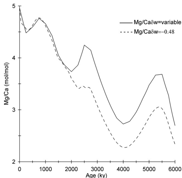
Fig. 1. Seawater Mg/Ca ( Mg/Ca_{sw} ) reconstructions by Fantle and DePaolo (2006) (FD06) (Fantle and DePaolo, 2006). These curves are based on two parameterizations of assumed \delta^{44}Ca value for weathering inputs to the ocean ( \delta_w ). In one case, it was assumed that the Ca isotopic composition of the weathering flux was constant ( \delta_w = -0.48\text{‰} ) over the past 20 Ma, whereas in the other case, the Ca isotopic composition of the weathering flux was constrained assuming that the ocean is in steady state over some time scale longer than 4 Ma ( \delta_w = \text{variable} ). The foraminiferal Mg/Ca-based SST records presented here were adjusted to account for past changes in seawater Mg/Ca using the curve that assumes variable \delta^{44}Ca weathering inputs to the ocean.
