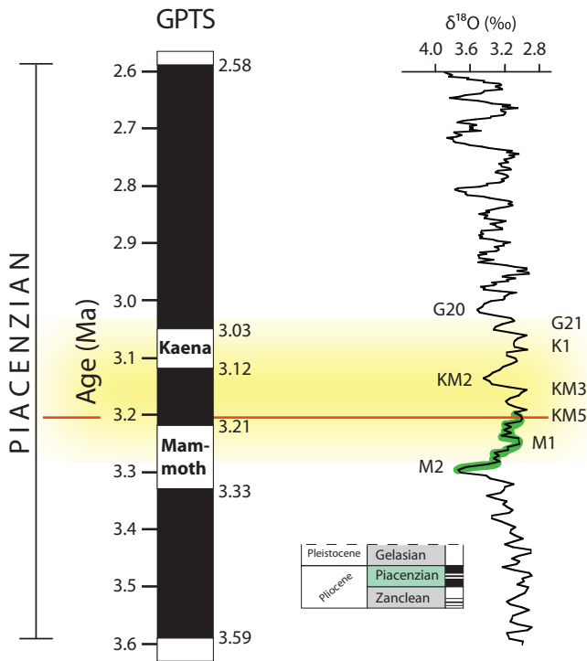
Figure 1. PRISM Pliocene magnetobiostratigraphic and stable isotopic framework. Benthic \delta^{18}\text{O} record from Lisiecki and Raymo (2005). Position of PRISM3 time slab (yellow band) and extent of PRISM4 time series (green highlighted section of LR04) between MIS M2 and MIS KM5. PlioMIP2 time slice (3.205 Ma) shown by horizontal red line. Magnetic polarity ages from Lourens et al. (1996).
