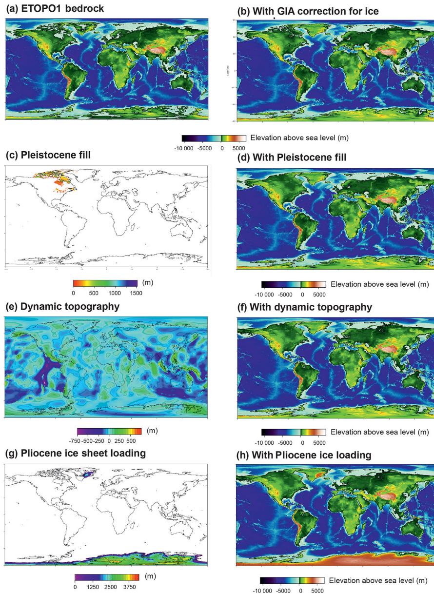
Figure 4. Generation of the PRISM4 paleogeography. Panel (a) shows “bedrock” (base of the ice sheets) version of ETOPO1 sampled at the working resolution of a quarter degree, (b) GIA correction, (c) Pleistocene landscape fill, (d) Pleistocene landscape features filled in, (e) dynamic topography correction, (f) dynamic topography correction applied to (d), (g) Piacenzian ice sheets, and (h) retrodicted PRISM4 paleogeography (g) applied to (f).
