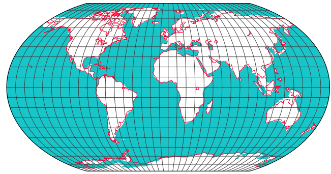
Figure 5. Pliocene sea level. Distribution of PRISM4 (Piacenzian) land area shown in white. Modern (ETOP01) coastline (red) for comparison.
