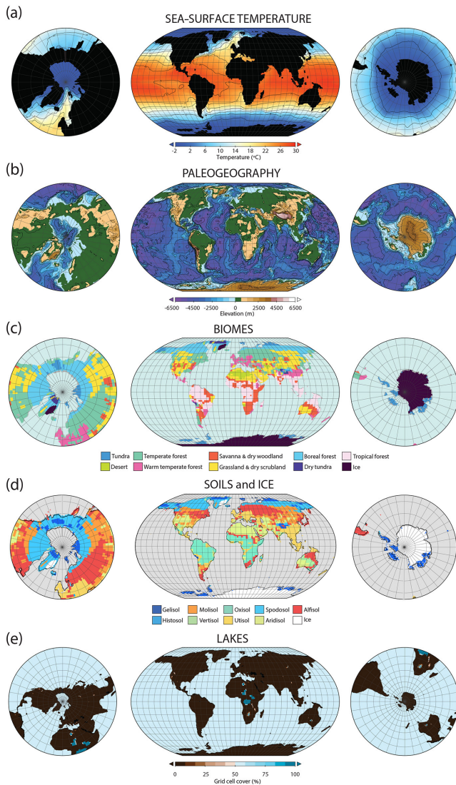
Figure 3. PRISM4 reconstruction. (a) Mean annual sea-surface temperature, (b) paleogeography, (c) biomes, (d) soils and land ice, and (e) large lakes.
