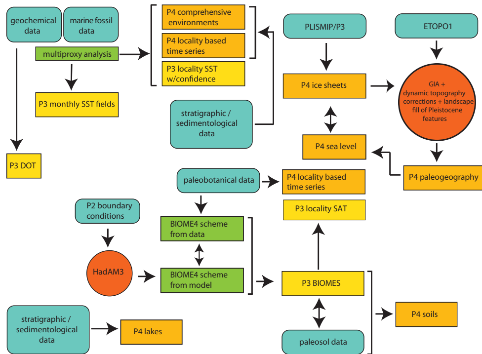
Figure 2. Interrelationships between PRISM3 and different parts of the PRISM4 reconstruction. Twelve data sets representing components of our Piacenzian reconstruction are shown in yellow and orange rectangles (PRISM3 and PRISM4, respectively). Starting points in the generation of these data sets are indicated by teal rounded rectangles. These are the basic geochemical, faunal, floral, soil, cryospheric, topographic, bathymetric, sedimentologic, and stratigraphic data. Marine temperature estimates (SST and DOT (deep-ocean temperature)) are based upon multiple proxies (including faunal, floral, geochemical, and biomarker analyses). Terrestrial vegetation data are translated into a BIOME4 scheme and compared to an independent BIOME4 landscape produced by the HadAM3/TRIFFID model (red circle) initialized with PRISM2 boundary conditions. Integration of data and model output results in the hybrid PRISM3 BIOME reconstruction (Salzmann et al., 2008). Antarctic and Greenland ice sheets are based upon PRISM3 and PLISMIP results, respectively. Paleogeography is based upon an initial ETOPO1 digital elevation model incorporating PRISM4 ice sheets, GIA, and adjustments due to mantle convection (red circle). Soils are determined through comparison of sedimentological and stratigraphic data with the PRISM3 BIOME reconstruction. Lakes are determined from stratigraphic and sedimentological data (Pound et al., 2014). Sea-level is estimated from the PRISM4 ice sheets and is consistent with the paleogeography presented here.
