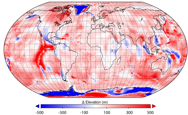
Figure 7. PRISM4 paleogeographic anomaly showing Piacenzian elevation (Fig. 4h) minus modern ETOPO1 (Fig. 4a) elevations (red positive, blue negative).
