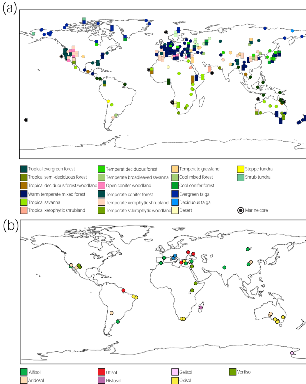
Figure 6. (a) Vegetation reconstruction for a cold/dry (upper square) and warm/wet (lower square) period of the Piacenzian (3.6–2.6 Ma). Circles show dominant Piacenzian biomes for each paleobotanical site. For a full explanation of methods and list of literature for each site, see Salzmänn et al. (2008, 2013). (b) Geographic distribution of Piacenzian soil localities used in the global reconstructions. Circles show the dominant soil type reconstructed from paleosol occurrences. For a full explanation of the method and list of literature for each site, see Pound et al. (2014).
