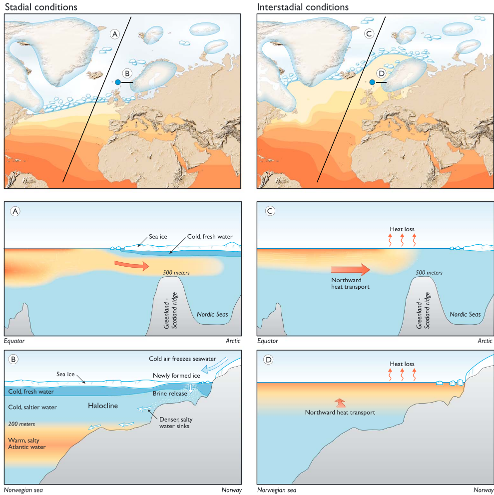
Figure 6. Schematic showing wintertime conditions in the North Atlantic and Nordic seas during typical cold stadal periods and (right) warm interstadial periods of a D-O cycle. (top) Maps of the North Atlantic region with sea ice extent and land ice. The location of the sediment core is marked with a blue dot, and the sections described in the bottom panels are indicated. (middle) locations A and C show north-south sections of the North Atlantic during stadial and interstadial conditions, respectively. (bottom) Locations B and D show east-west sections of the Norwegian Sea during stadial and interstadial conditions, respectively.
