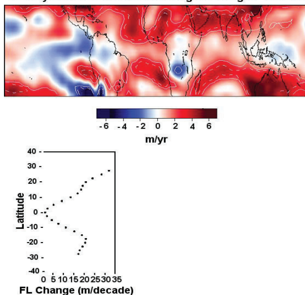
FIGURE 3. Changes in tropical freezing level heights for the period 1977–2007 (top panel) and profile of zonally averaged values (bottom panel). After Bradley et al. (2009).
