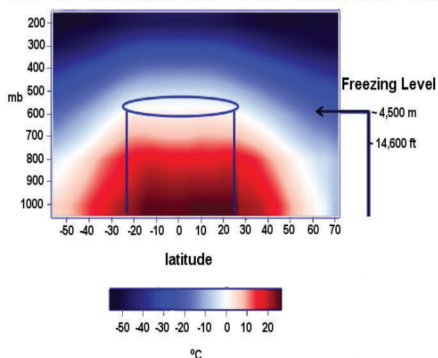
FIGURE 2. The distribution of mean free air temperature (°C) in the atmosphere (1973–2002) based on NCEP reanalysis. Freezing level height occurs at ~4500 m in the tropical belt.
