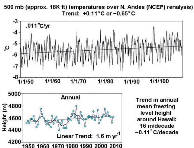
FIGURE 12. Comparison of (top panel) 500 mb air temperature for the northern Andes (cf. Fig. 8), and (bottom panel) the rise in freezing level height in Hawai'i. Temperature changes in both regions at approximately equal altitudes are very similar. Bottom panel is taken from Diaz et al. (2011).
