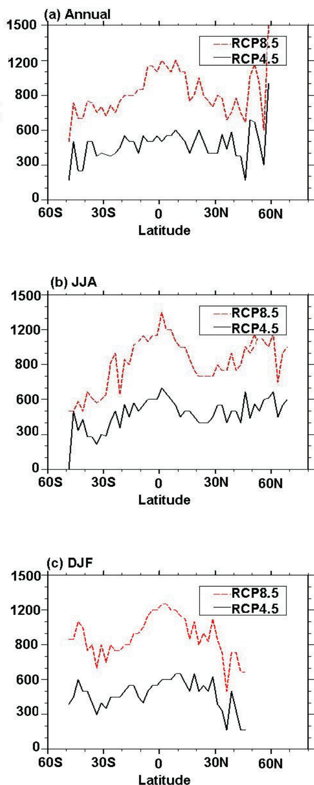
FIGURE 11. The differences between historical and future freezing elevations on (a) annual, (b) boreal summer, and (c) boreal winter under the RCP4.5 (solid curves) and RCP8.5 (dashed curves) scenarios. Differences are calculated for the period 2081–2100 minus 1981–2000.
