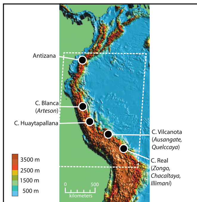
Fig. 1. Map of the tropical Andes, with locations of glaciers and mountain ranges discussed in the text. White box ( 2^{\circ}\text{N} – 18^{\circ}\text{S} / 65^{\circ} – 82^{\circ}\text{W} ) indicates area over which CMIP 5 models were averaged to derive simulated historical and projected temperature change over the Andes.
