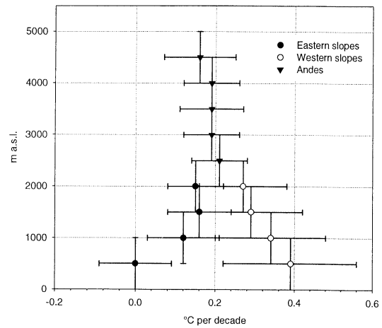
Figure 4. Temperature trend (°C/decade) as a function of elevation (m a.s.l.). Vertical bars indicate elevation range ( \pm 500 m) for which trend is valid. Horizontal bars are 95% confidence limits for the trend and extend two standard errors of estimate on either side (i.e. all trends whose horizontal bars
