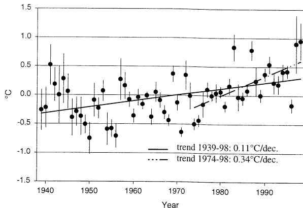
Figure 3. Annual temperature deviation from the 1961-1990 average in the tropical Andes (1°N-23°S) between 1939 and 1998. Trend estimates are based on ordinary least squares (OLS) regression. Vertical bars extend 2 standard errors of the mean either side of the annual average.
