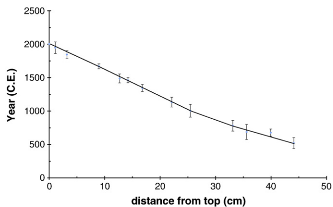
Fig. 2. Chaac ^{230}\text{Th} age model. The blue squares represent ^{230}\text{Th} ages with errors between 38 and 112 years (Supplementary Table S1). The chronology is based on a piece-linear model. Linear interpolation was performed between ^{230}\text{Th} dates in the following depth intervals (cm from the top): 44.1–33.1 [Year (C.E.) = -23.64 * \text{distance (cm)} + 1563 ], 33.1–25.45 [Year (C.E.) = -29.214 * \text{distance (cm)} + 1747.9 ], 25.45–8.95 [Year (C.E.) = -40.331 * \text{distance (cm)} + 2030.8 ], and 8.95–top [Year (C.E.) = -38.914 * \text{distance} + 2004 ].
