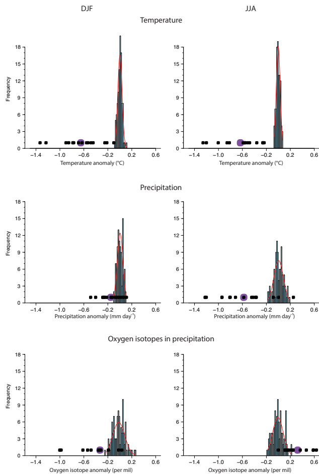
Figure 12. Frequency distribution of 100 random 45-event composites in LM control simulation of ModelE2-R (blue) for temperature (top row), precipitation (middle), and oxygen isotopes in precipitation (bottom) for DJF (left column) and JJA (right column). Results averaged over same domains as in Fig. 9. Normal distribution with a mean and standard deviation equal to that of the data shown in red. Purple square shows the single 45-event composite used in this study, with the distribution of individual 15 volcanic eruptions (each averaged over three ensemble members) in black dots.
