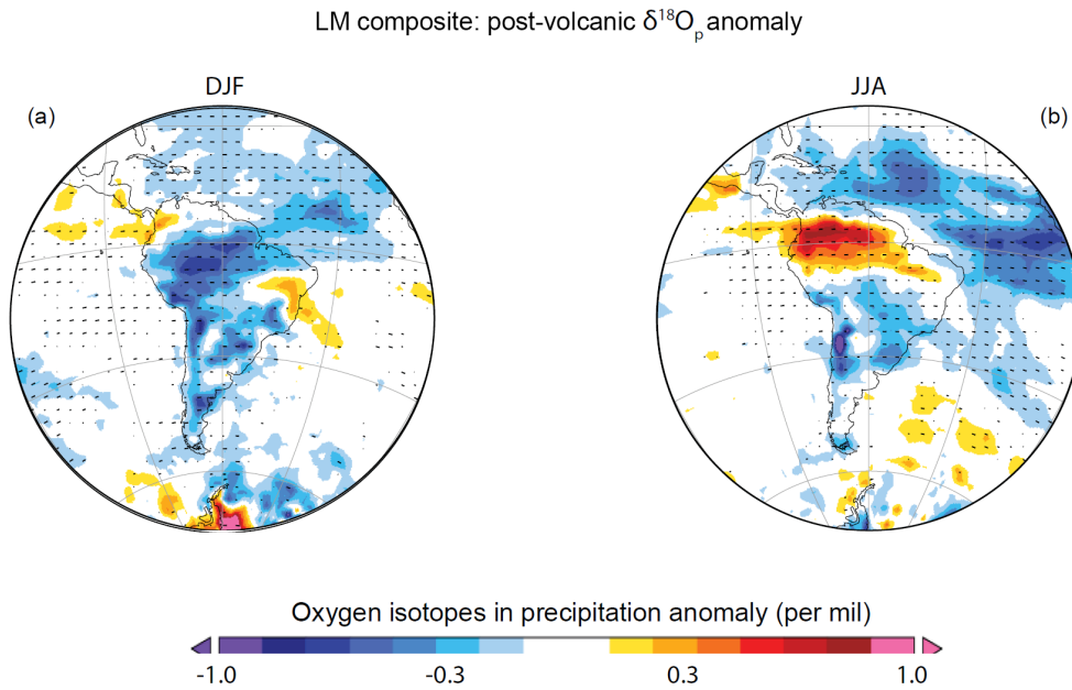
Figure 10. Last millennium post-volcanic oxygen isotope in precipitation ( \Delta\delta^{18}\text{O}_p ) composite (per mil) with all eruption events during (a) DJF and (b) JJA from GISS ModelE2-R using procedure described in the text. Stippling highlights areas with anomalies significant at p < 0.1 .
