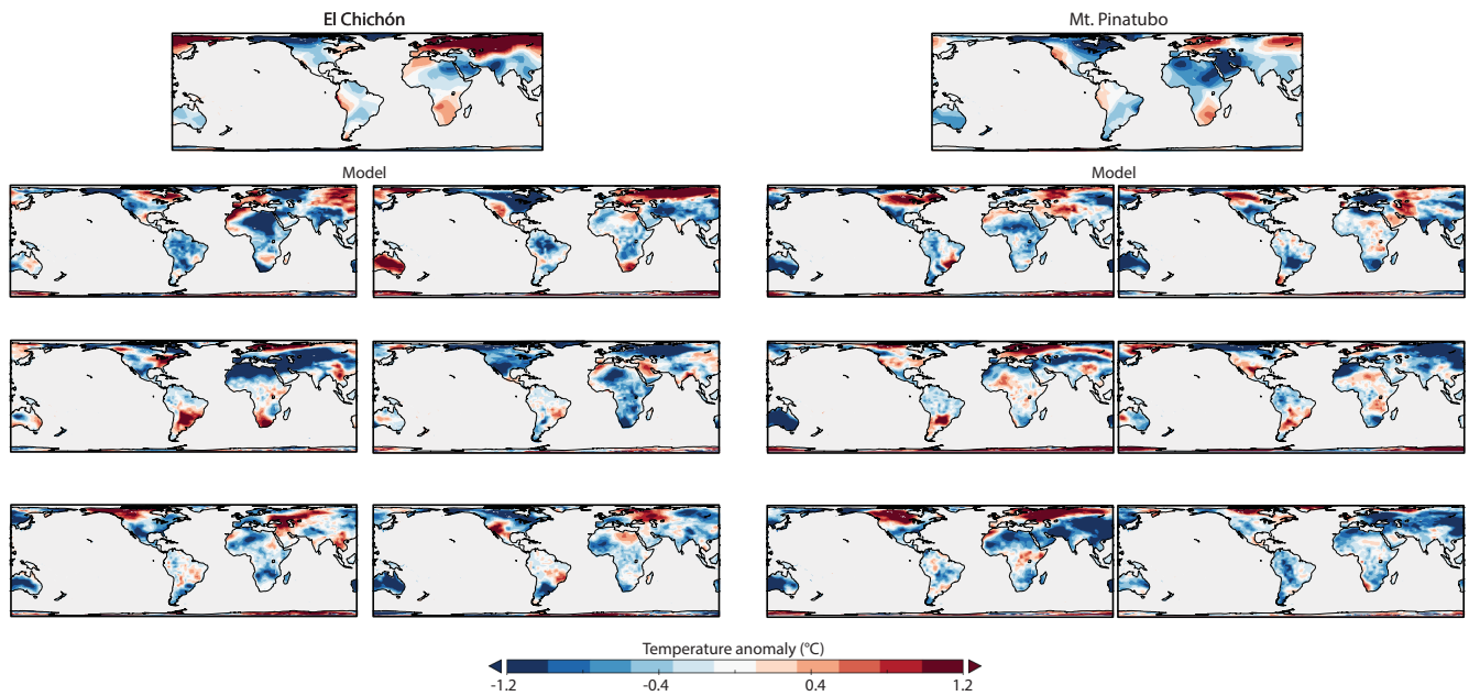
Figure 5. Annual-mean temperature change ( ^{\circ}\text{C} , ocean masked) for each L20 eruption (labeled on plot) in GISTEMP (top row) and each ModelE2-R ensemble member, as discussed in the text. All plots use ENSO-removal procedure described in the text.
