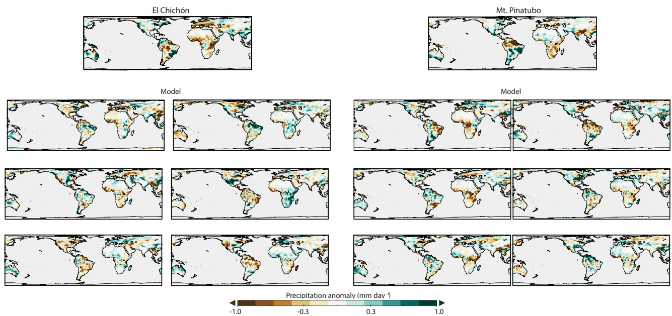
Figure 6. As in Fig. 5, except for precipitation change ( \text{mm day}^{-1} ).
