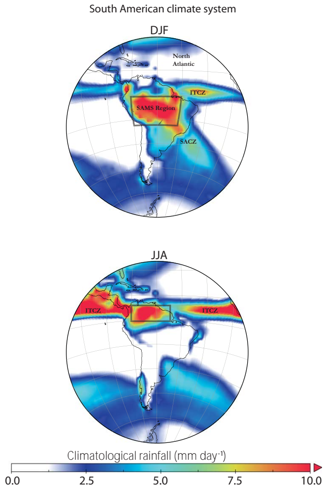
Figure 2. Top: observed Climatological Precipitation for DJF (shading, in \text{mm day}^{-1} ). SAMS box is drawn over the domain from 20 to 0°, 77.5 to 45° W and used for Figs. 9 and 12. Data from the GPCP product, long-term climatological rainfall derived from years 1981–2010. Bottom: as above, except for JJA. Box from 0 to 10° N, 77.5 to 52.5° W used in averaging for Figs. 9 and 12.
