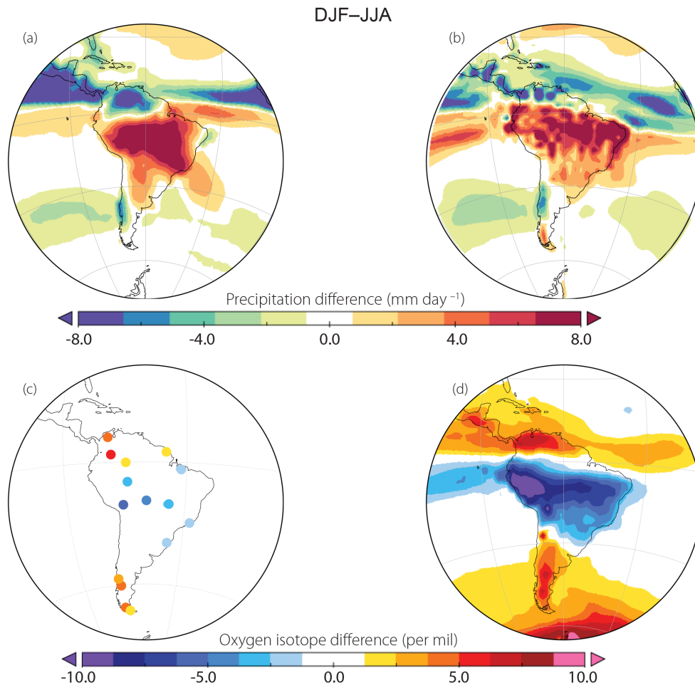
Figure 3. Seasonal cycle (DJF minus JJA) of precipitation in the (a) GPCP precipitation product, from data in Fig. 2, (b) in ModelE2-R, (c) \delta^{18}\text{O}_p in GNIP data, and (d) \delta^{18}\text{O}_p in ModelE2-R. GNIP data only shown for stations with at least 90 reported \delta^{18}\text{O}_p values at a given station from 1960 to present, in addition to at least 10 data values for each month: December, January, February, June, July, and August. Stations with seasonal differences of less than \pm 1.0\text{‰} are also omitted in panel (c).
