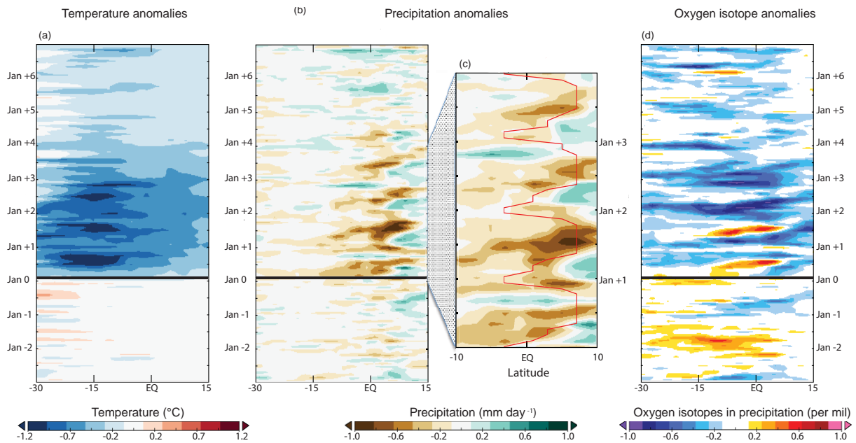
Figure 11. Last millennium Hovmöller diagram (10 years, time moving forward going upward, with year number labeled next to each month) for (a) temperature anomaly ( ^{\circ}\text{C} ) and (b) precipitation anomaly ( \text{mm day}^{-1} ) using procedure described in the text. Solid black lines mark closest January to start of each eruption used in composite. (c) Same as panel (b), except zoomed in on 10^{\circ}\text{S} to 10^{\circ}\text{N} and over 3 years of time beginning with the January closest to each eruption. Red line in panel (c) shows latitude of maximum climatological precipitation as a function of time of year. All results zonally averaged in model from 77.5 to 45^{\circ}\text{W} . (d) Last millennium Hovmöller diagram for oxygen isotopes in precipitation (per mil).
