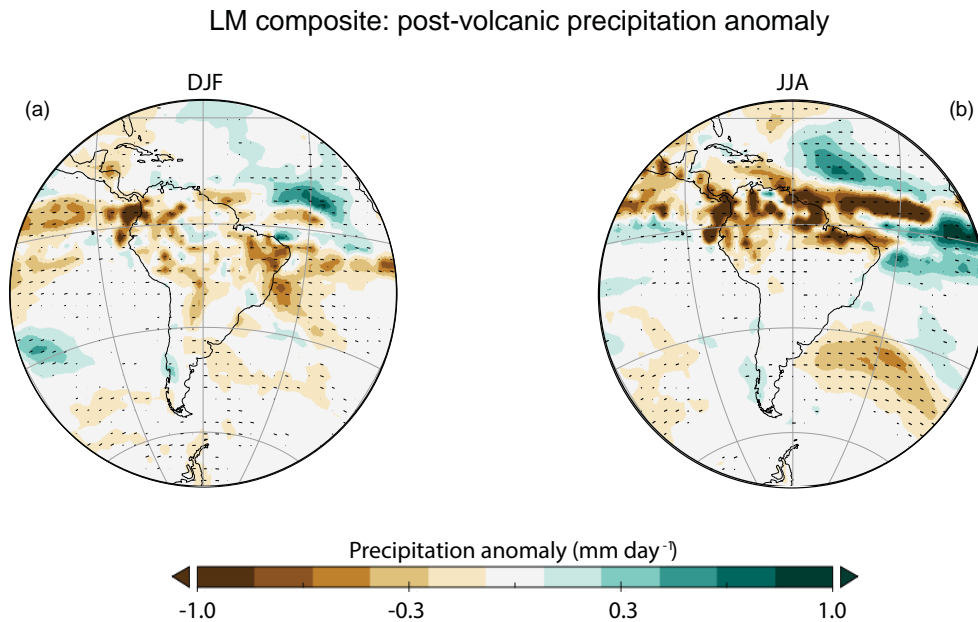
Figure 8. Last millennium post-volcanic precipitation composite ( \text{mm day}^{-1} ) with all eruption events during (a) DJF and (b) JJA from GISS ModelE2-R using procedure described in the text. Stippling highlights areas with anomalies significant at p < 0.1 .
