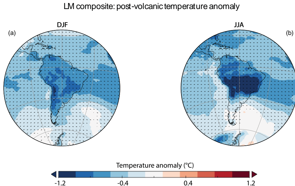
Figure 7. Last millennium post-volcanic temperature composite ( ^{\circ}\text{C} ) averaged over all 45 events during (a) DJF and (b) JJA from GISS ModelE2-R using procedure described in the text. Stippling highlights areas with anomalies significant at p < 0.1 .
