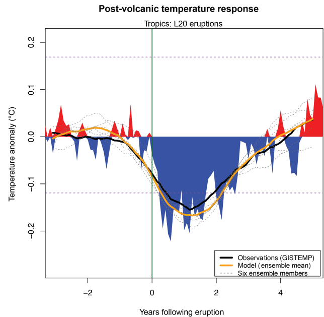
Figure 4. Composite tropical ( 30^{\circ}\text{S} to 30^{\circ}\text{N} ) temperature response following the L20 volcanic eruptions. Fill colors denote observed monthly anomalies using GISTEMP, with 24-month running average shown as a solid black line. ModelE2-R ensemble mean is shown as solid orange line and dashed grey lines indicate the six individual ensemble members. Anomalies are referenced to 5 years prior to eruptions (years -5 to 0 ). Dashed purple lines encompass the 5–95 % interval for monthly tropical-mean temperature anomalies (relative to the previous 5-year mean) in the GISTEMP product from 1950 to present. The calculation of this range omits data 2 years after the L20 eruptions. The range is not symmetric about zero due to the tropical warming trend during this interval. All data are based on the ENSO-removal technique discussed in the text.
