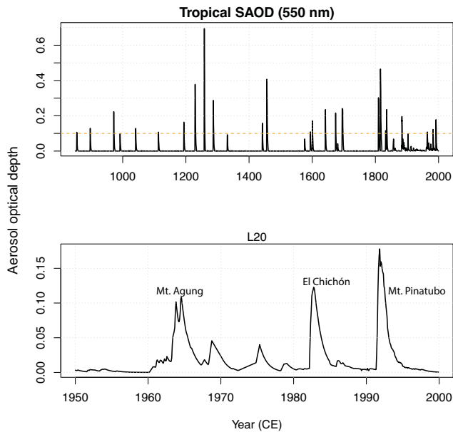
Figure 1. Aerosol optical depth (AOD) used to force the NASA GISS ModelE2-R over the last millennium and (bottom) zoomed in on the period 1950–1999 (Sato et al., 1993; Crowley and Unterman, 2013) as discussed in the text. AOD is the vertically integrated (15–35 km) and latitudinal average from 30° S to 30° N. Note difference in vertical scale between graphs. Orange dashed line marks the AOD threshold for defining a LM eruption in the present study. Eruption events defined in the text must sustain the threshold AOD for at least 1 year, so not all events above the orange dashed line are used in the composites.
